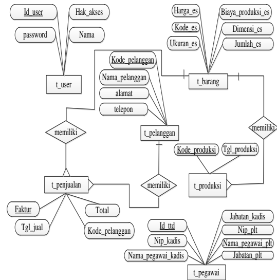
Gambar 6. Entity Relationship Diagram(ERD)
