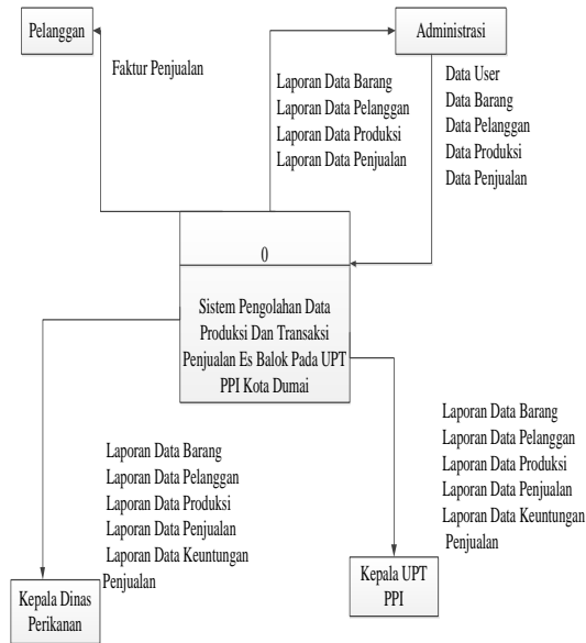
Gambar 4. Context Diagram
